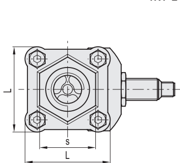
HVF-E (G3/4 - G1)
