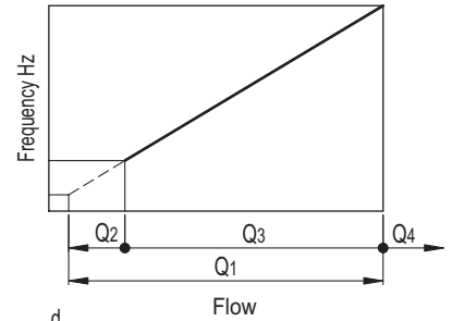
HVF-E (G3/8 - G1/2)
